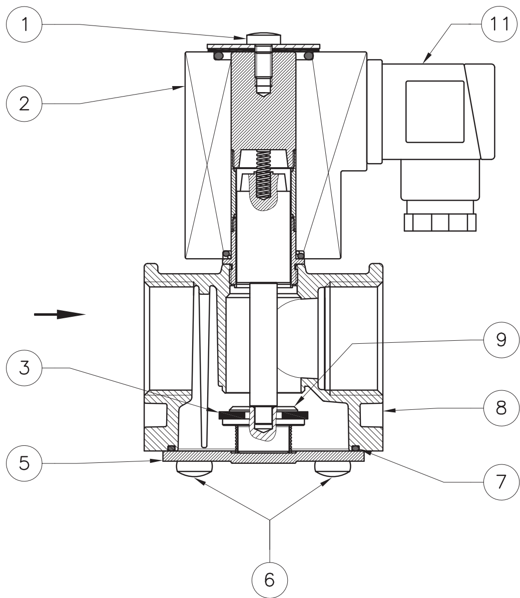
fig. 2 (EVAP-1-3-6/NA - DN 15 ÷ 25)
